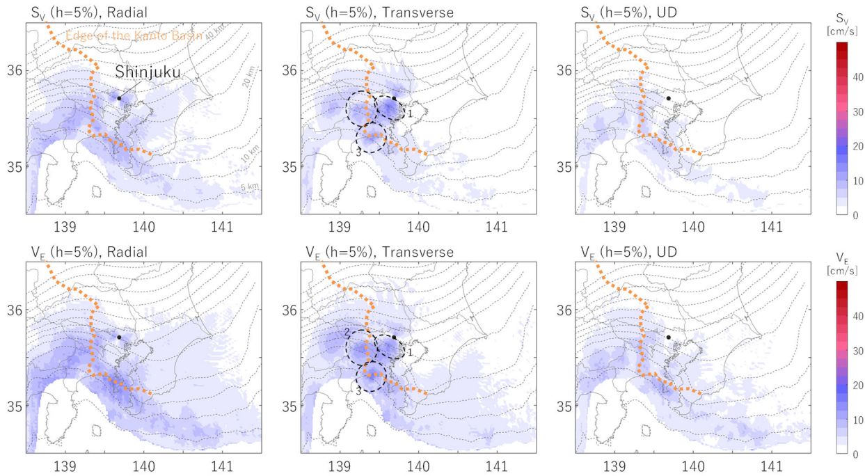
Fig. 4 – Results for rake angle of 0^\circ ; the damping constant was set at 5%.
