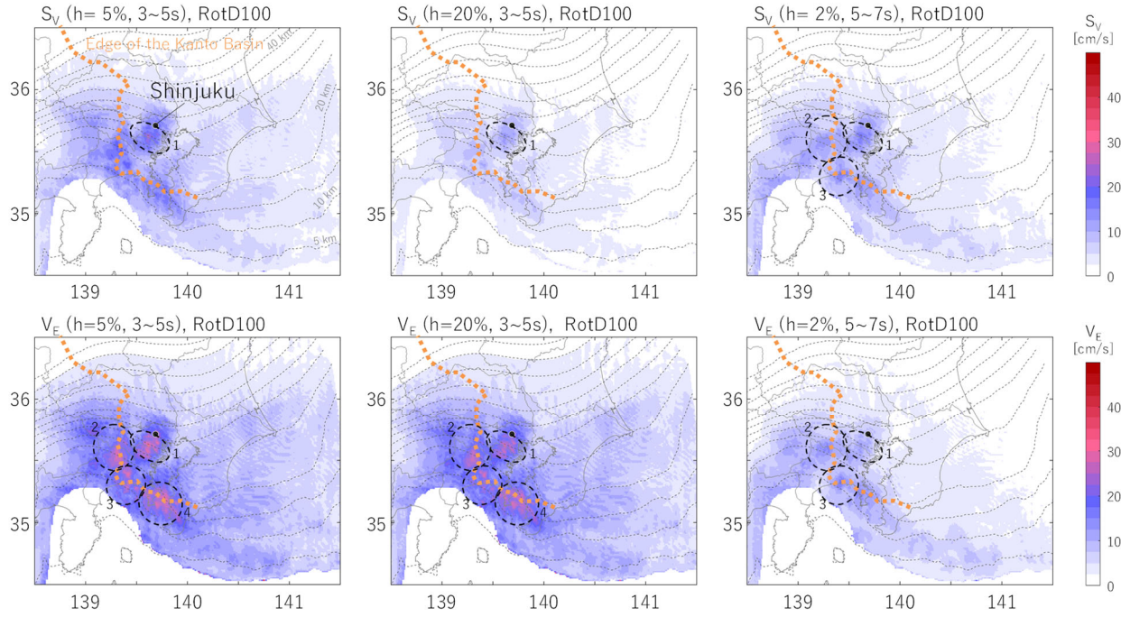
Fig. 6 – Difference as per building type. From left: Damping building (3 - 5 s, h = 5\% ), seismic isolated building (3 - 5 s, h = 20\% ), and super high-rise building (5 - 7 s, h = 2\% ). The value to plot is RotD100. Results of rake angle 0^\circ are shown.
