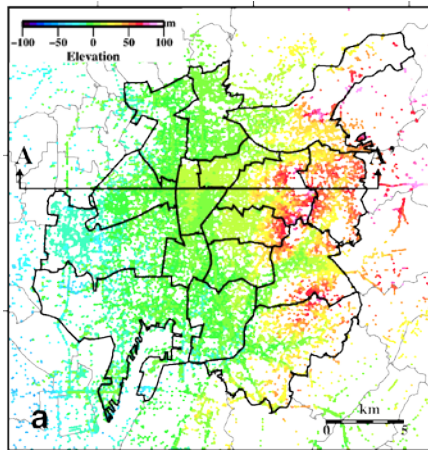
Fig. 4 – The distribution of the lower elevation of the AO layer from borehole logs (a), from the geotechnical engineering maps [1] (b) and from interpolated grid (c).
