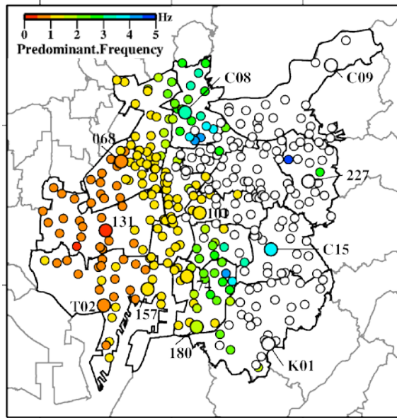
Fig. 8 – The distribution of predominant frequency based on the microtremour records.
