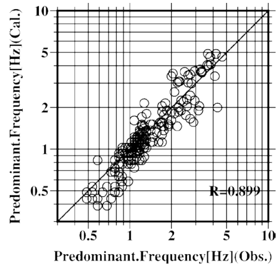
Fig. 10 – Comparison with the predominant frequency of the observed H/V spectra and that of the theoretical H/V spectra.
