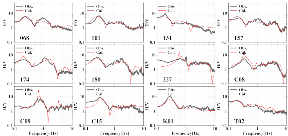
Fig. 9 – Examples of comparison between theoretical H/V spectra and observed H/V spectra based on microtremour
