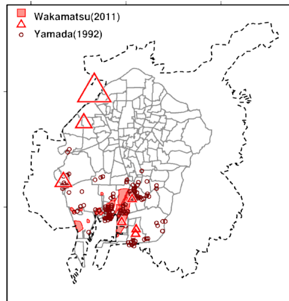
Fig. 15 – The distribution of liquefaction areas due to Tonankai earthquake in 1944.
