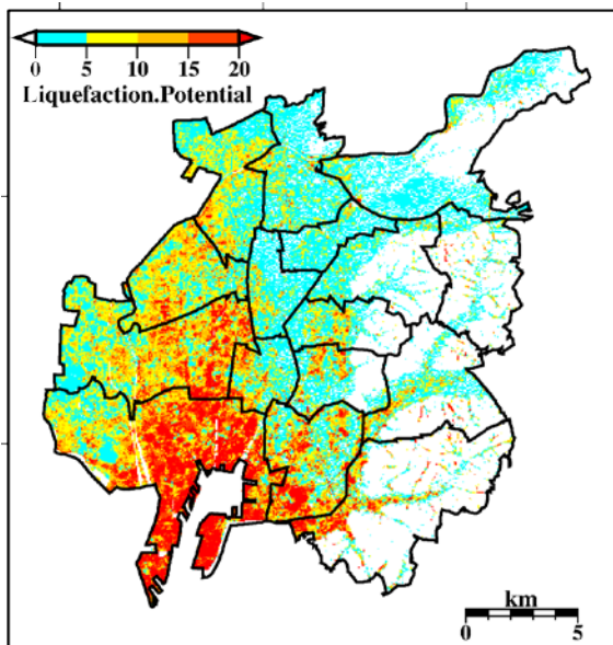
Fig. 14 – The distribution of PL-value.
