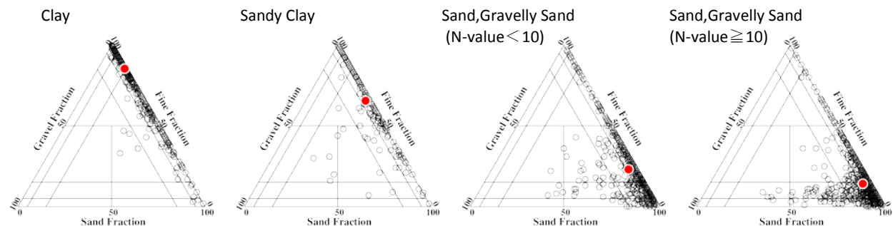
Fig. 5 –The grain size distribution is shown for each index of lithofacies in triangular coordinates as an example.
