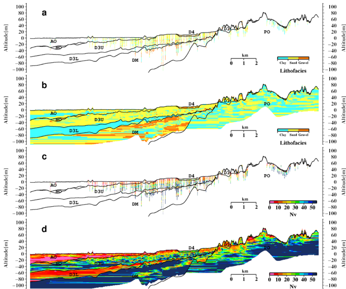
Fig. 6 – Borehole logs projected to A-A' line in the Fig.1 (a : lithofacies, c : N-values), and a cross section of lithofacies (b) and N-values (d) from constructed 3D models.
