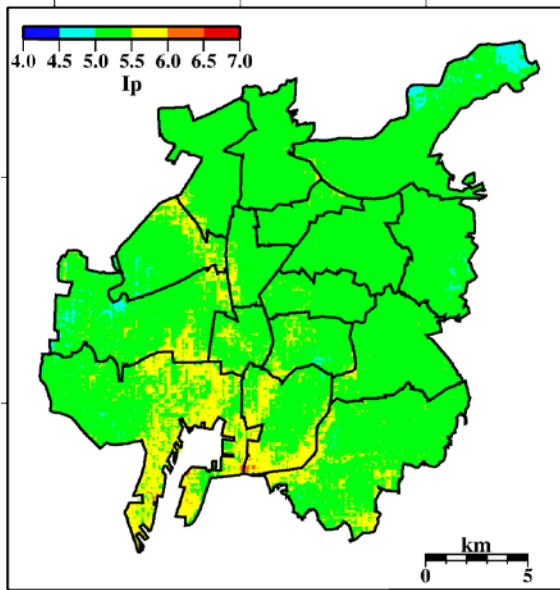
Fig. 12 – The distribution of simulated I_p .
