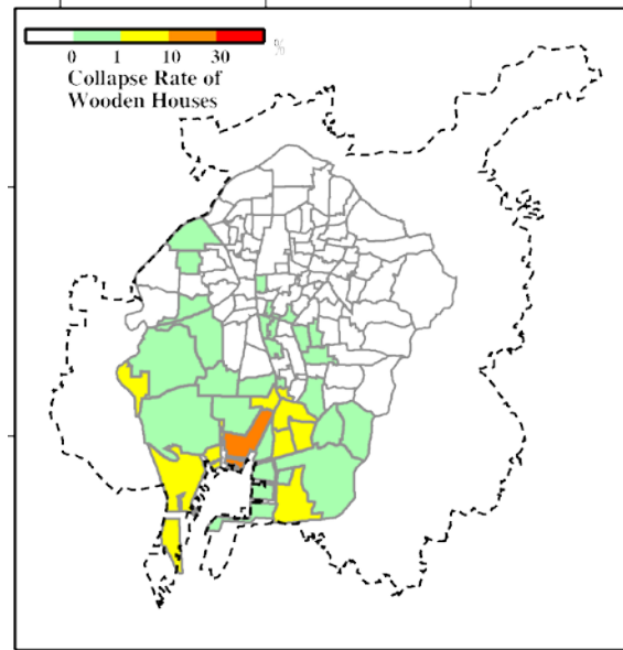
Fig. 13 – The distribution of collapse rate of wooden houses due to Tonankai earthquake in 1944.
