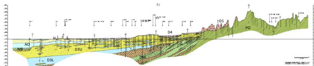
Fig. 7 – The geological profile from geotechnical engineering maps [1].
