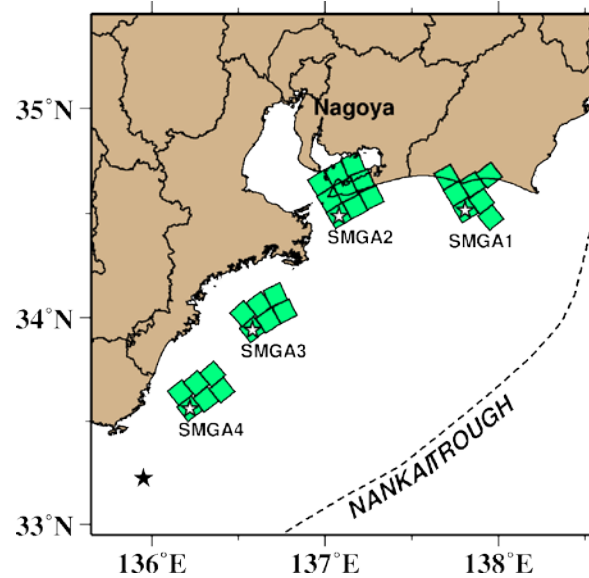
Fig. 11 – The source model of the hypothetical Tonankai earthquake [8]
