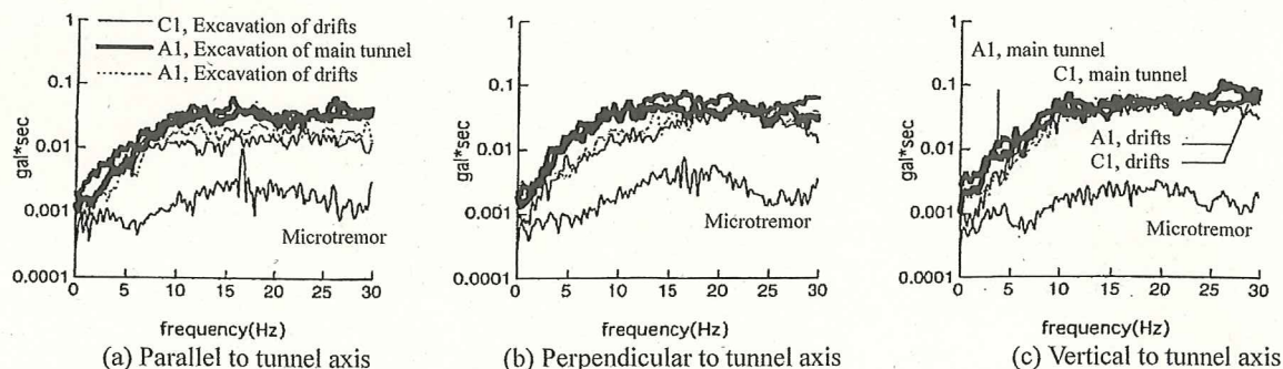
Fig.4. Acceleration Spectra during Excavation of Drifts and Main Tunnel Measured at Transects A (A1) and C (C1)
