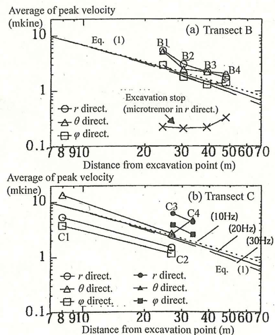
Fig.7. Attenuation of Maximum Vibration Amplitude with Distance on Transects B & C
