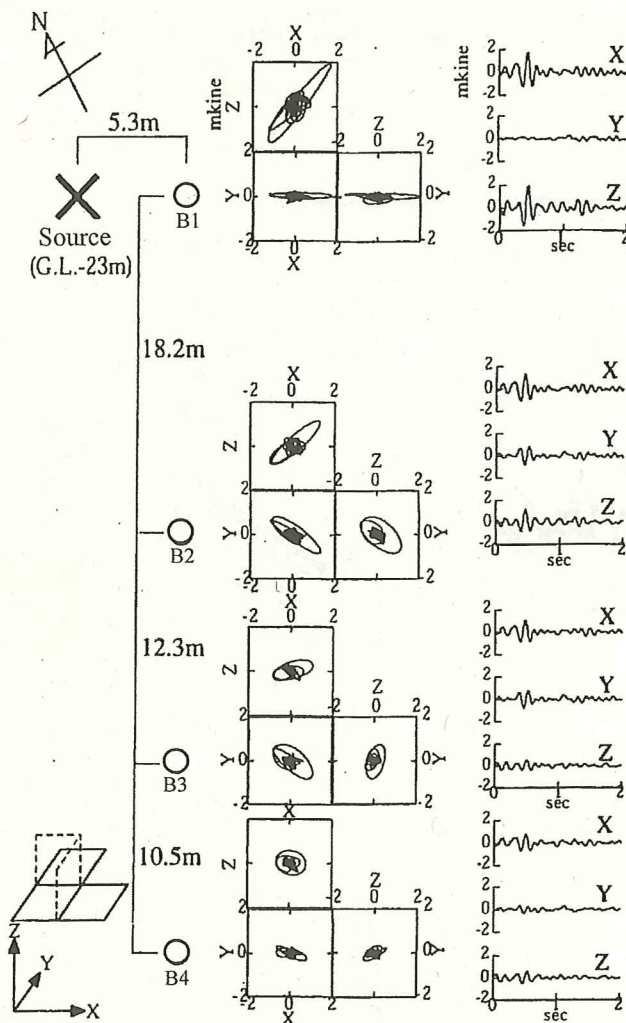
Fig.5. Three-dimensional Particle Motion of Observation Points on Transect B
