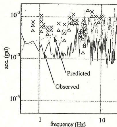
Fig.11. Predicted and Observed HVEM Acceleration Spectra during Closest Approach of Digging Operation
