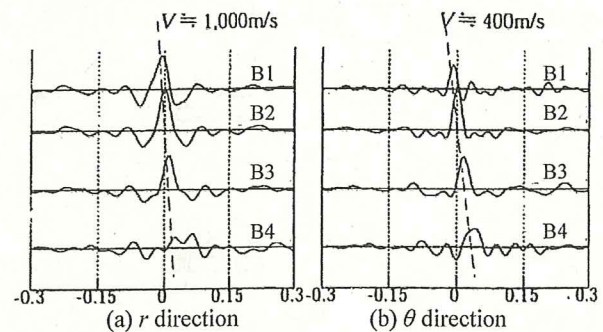
Fig.6. Cross Correlation Functions along Transect B
