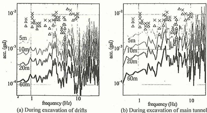
Fig.10. Level of Interference due to Acceleration of the HVEM ( \times : Clear Interference : \Delta Not Clear) and Predicted Acceleration Spectra for Distance from Operations
