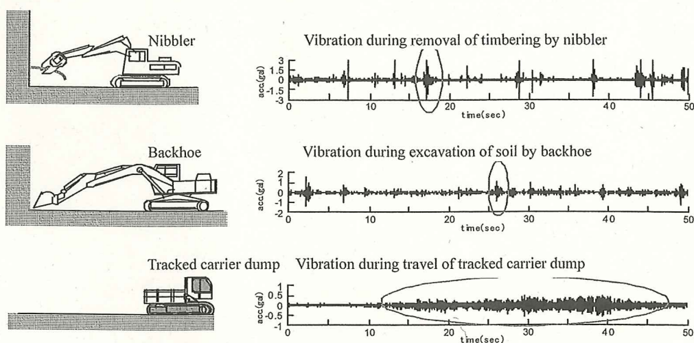
Fig.2. Characteristics of Vibration caused by Different Construction Equipment
