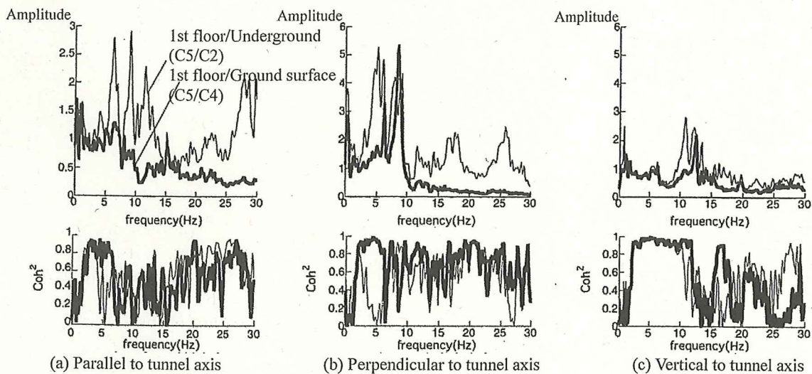
Fig.8. Transfer Functions and Coherences Concerning Building Containing HVEM
