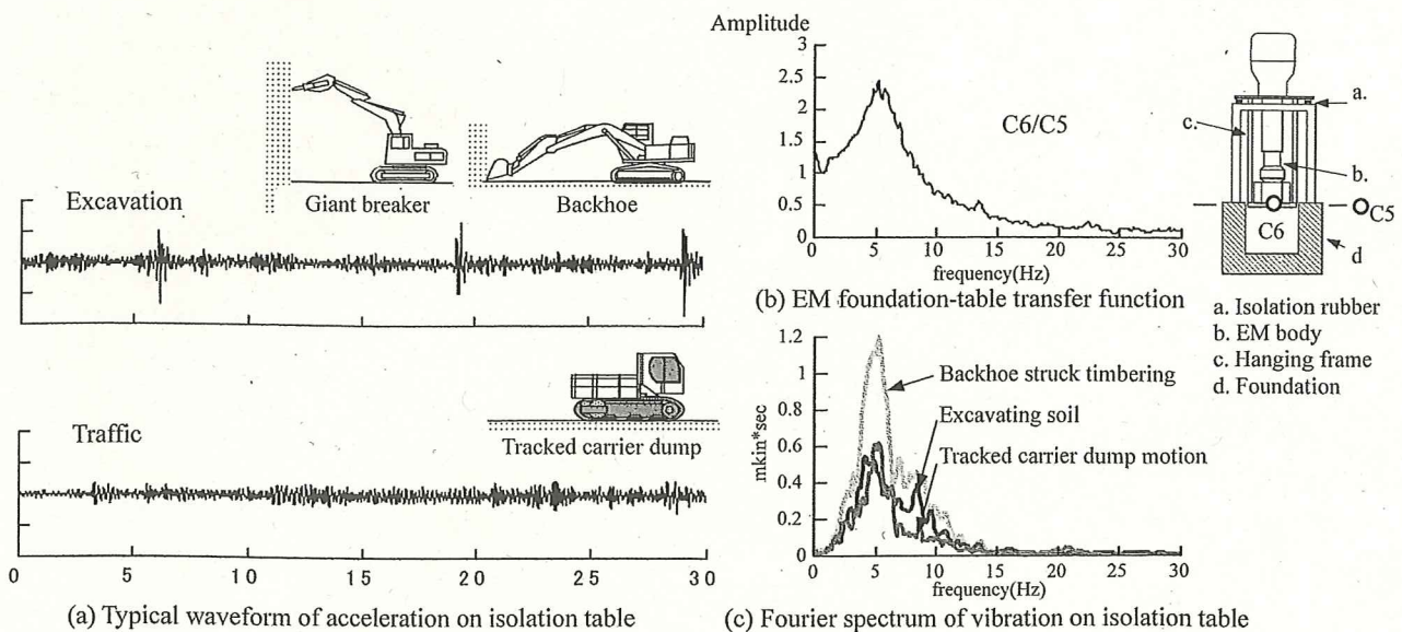
Fig.9. Vibrations Experienced by the HVEM Installed on an Isolation Table
