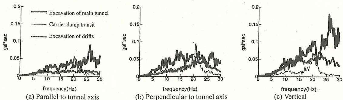
Fig.3. Acceleration Spectra during Equipment Operation along Transect A (Sensor A1)
