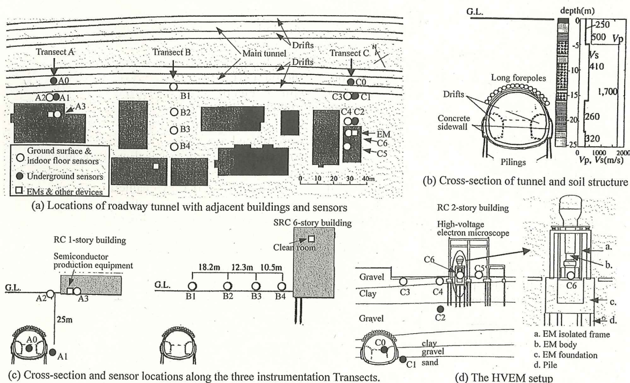
Fig.1. Outline of the Tunnel Project, Nearby Buildings, HVEM Setup, and the Sensor Networks
