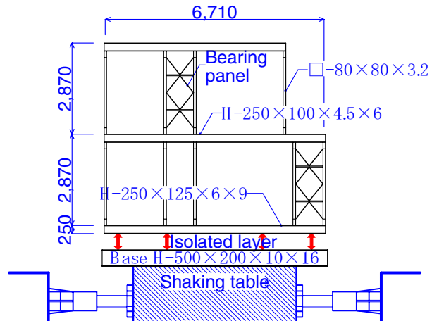
Fig.1. Test section
