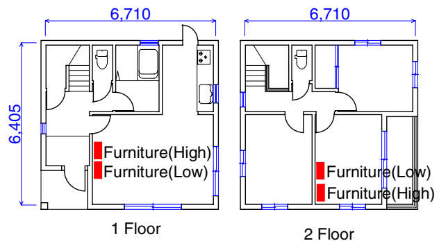
Fig.2. Test plan
